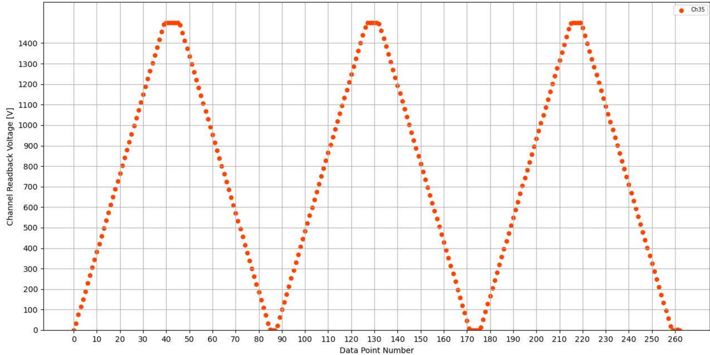
Voltage Ramp Test (Python) Bd #337, Slot #12, Ch #35
